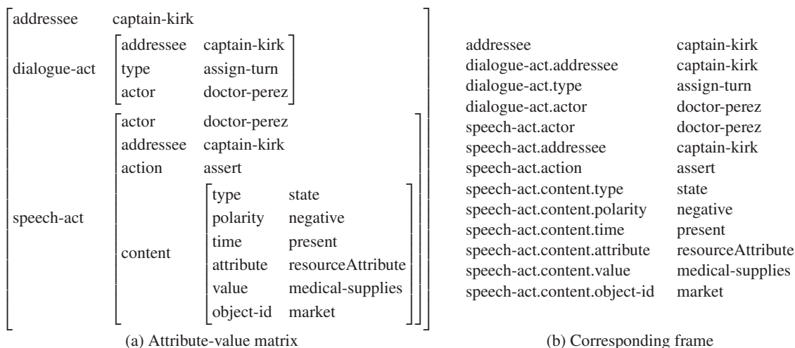
Figure 2: An example of Doctor Perez’s representations for utterance semantics: Doctor Perez tells the captain that there are no medical supplies at the market.
